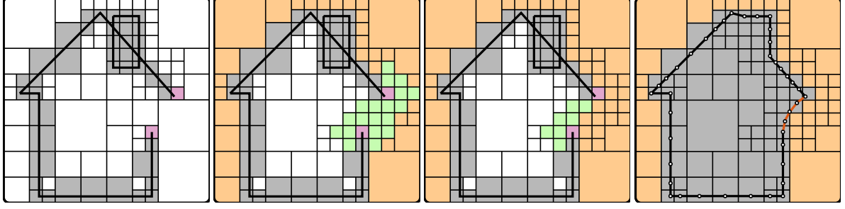
Figure 16: Left: Adaptive octree, boundary cells are marked red. Center left: Dilated boundary (green) and outside component (orange). Center right: Outside component dilated back into the boundary cells. Right: Final reconstruction
