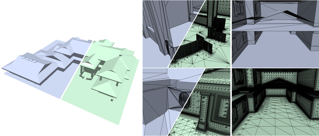
Figure 15: Reconstruction (green) of a triangle soup (blue). Left: Visually there is no difference between the triangle soup and the reconstruction. Middle: The reconstruction is a watertight mesh that is refined near the model features. Right: The volumetric approach allows to reliably detect and remove excess interior geometry from the input.
