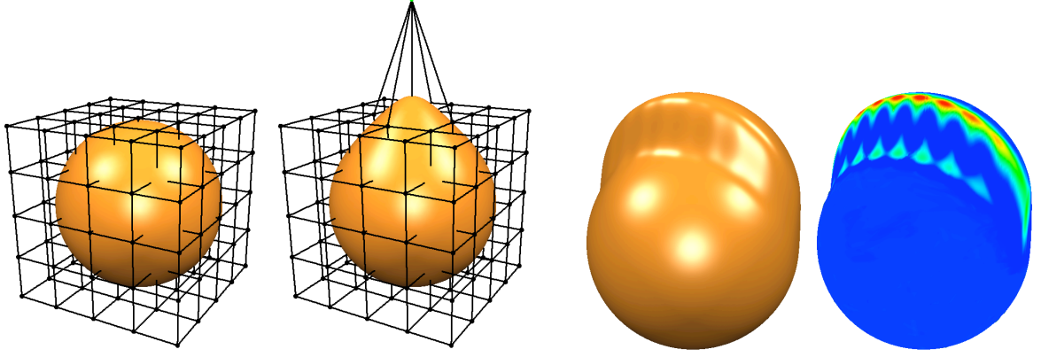
Figure 46: In the freeform deformation approach a regular 3D control lattice is used to specify a volumetric displacement function (left). Similar to tensor-product spline surfaces, the tri-variate tensor-product splines can also lead to alias artifacts in the deformed surface (right).
