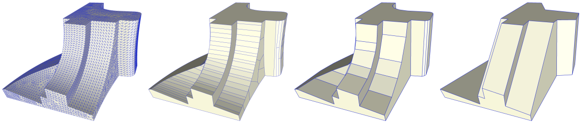
Figure 39: A multi-resolution hierarchy of differently detailed meshes that was created by variational shape approximation.
