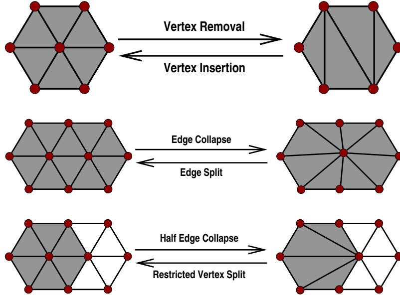
Figure 34: Euler-operations for incremental mesh decimation and their inverses: vertex removal, full edge collapse, and half-edge collapse.
