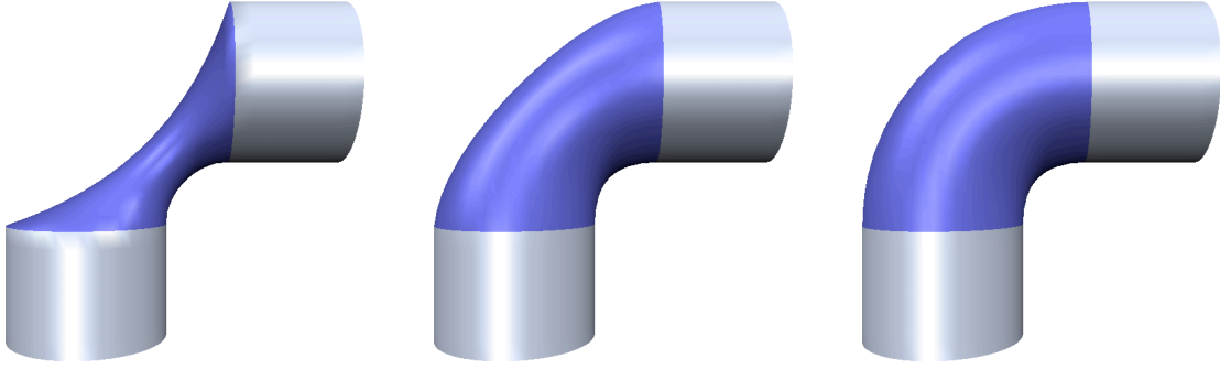
Figure 26: The order k of the energy functional and of the corresponding Euler-Lagrange PDE \Delta_S^k \mathbf{x} = 0 defines the stiffness of the surface in the support region and the maximum smoothness C^{k-1} of the boundary conditions. From left to right: membrane surface ( k = 1 ), thin-plate surface ( k = 2 ), minimum variation surface ( k = 3 ).
