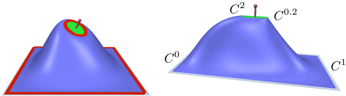
Figure 44: Minimizing the thin-plate energy allows for C^1 boundary constraints, which are given by the first two rings of fixed and handle vertices (left). The framework even allows for anisotropic bending behavior and per-vertex control of boundary continuity (right).
