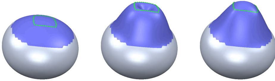
Figure 43: A sphere is deformed by lifting a closed handle polygon (left). Propagating this translation based on geodesic distance causes a dent in the interior of the handle polygon (center). The more intuitive solution of a smooth interpolation (right) cannot be achieved with this approach; it was produced by boundary constraint modeling.
