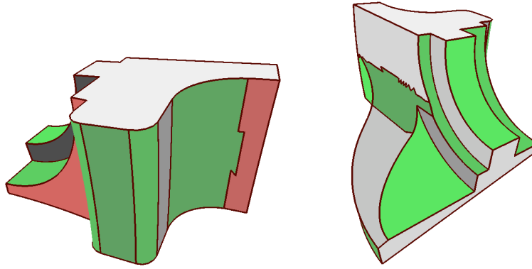
Figure 40: Hybrid Variational Surface Approximation: In addition to planes, Wu and Kobbelt also use more general proxies like spheres, cylinders, and rolling ball blends. These proxies allow to recover the semantic structure of the input model.
