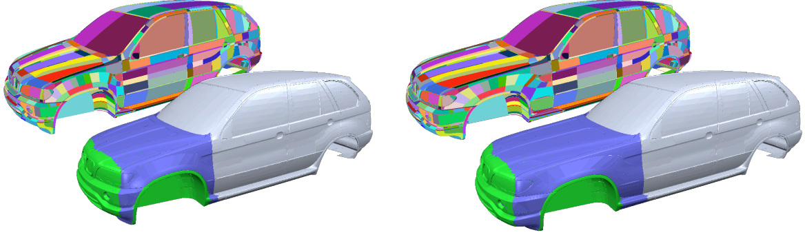
Figure 47: Using multiple independent handle components allows to stretch the hood while rigidly preserving the shape of the wheel houses. This 3M triangle model consists of 10k individual connected components, which are neither two-manifold nor consistently oriented.
