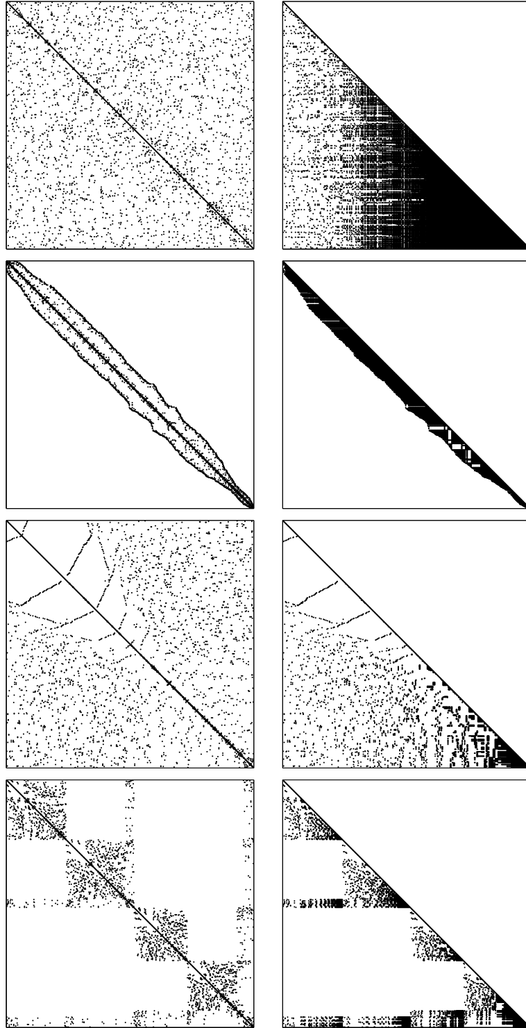
Figure 55: The top row shows the non-zero pattern of a typical 500 \times 500 matrix \mathbf{A} and its Cholesky factor \mathbf{L} , corresponding to a Laplacian system on a triangle mesh. Although \mathbf{A} is highly sparse (3502 non-zeros), the factor \mathbf{L} is dense (36k non-zeros). The reverse Cuthill-McKee algorithm minimizes the envelope of the matrix, resulting in 14k non-zeros of \mathbf{L} (2nd row). The minimum degree ordering avoids fill-in during the factorization, which decreases the number of non-zeros to 6203 (3rd row). The last row shows the result of a nested dissection method (7142 non-zeros), that allows for parallelization due to its block structure.
