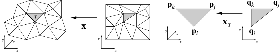
Figure 28: Example of a piecewise linear mapping. The meshes share the same connectivity, and individual triangles are mapped.
