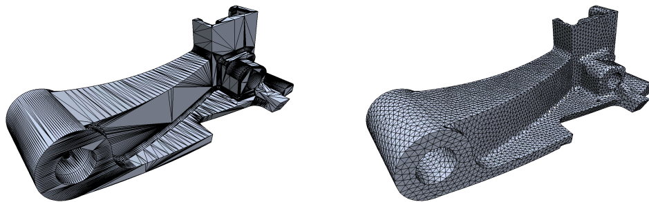
Figure 37: Isotropic, feature sensitive remeshing of a CAD model.
