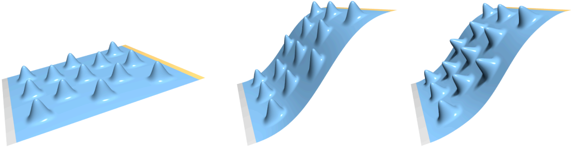
Figure 48: Fine-scale surface details are distorted by freeform deformations due to the lack of local frame rotations. For this pure translation, all surface points move in the same direction. In contrast, multiresolution deformations correctly preserve the bumps under global deformations.
