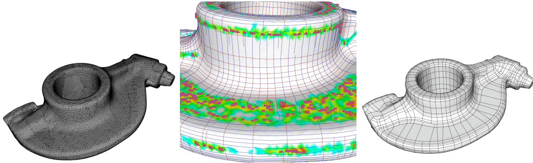
Figure 38: Quad-dominant remeshing. Left: The input is a manifold triangle mesh. Middle: In regions of low confidence, the curvature lines are not well-defined. The algorithm bridges these regions by extrapolation and produces the result on the right.
