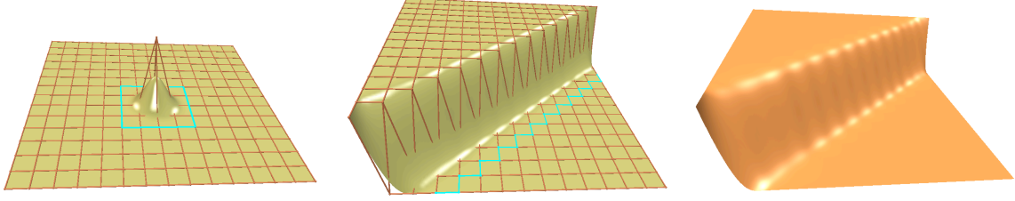
Figure 41: A modeling example using a bi-cubic tensor-product spline surface. Each control point is associated with a smooth basis function of fixed rectangular support (left). This fixed support and the fixed regular placement of the control points, resp. basis functions, prevents a precise support specification (center) and can lead to alias artifacts in the resulting surface, that are revealed by more sensitive surface shading (right).
