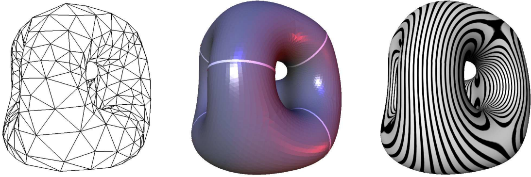
Figure 27: Six circles with C^1 boundary-conditions are used to design a “tetra thing”. Due to the symmetry the final solution is actually G^2 continuous in this case, which is indicated by the smooth reflection lines (see Chapter 6). Surfaces are constructed using the intrinsic fairing method [SK01] based on solving \Delta_S H = 0 , therefore the solution is independent of the triangulation (or parameterization, respectively).
