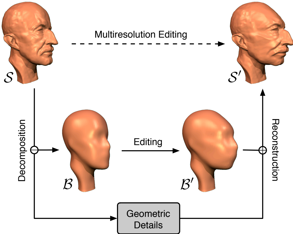
Figure 11.10: A general multiresolution editing framework consists of three main operators: the decomposition operator, that separates the low and high frequencies, the editing operator, that deforms the low frequency components, and the reconstruction operator, that adds the details back onto the modified base surface. Since the lower part of this scheme is hidden in the multiresolution kernel, only the multiresolution edit in the top row is visible to the designer.
