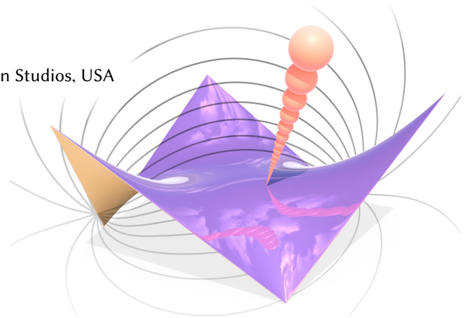
Fig. 1. We introduce a ray tracing algorithm for a novel class of surfaces defined by level sets of harmonic functions. Here for instance we directly visualize a nonplanar polygon which has no well-defined inside or outside—and hence cannot be represented by an ordinary implicit function or SDF. Isolines depict a 2D slice of the harmonic function; spheres show conservative Harnack bounds along a ray. Note the smooth reflection lines, even near edges and vertices where the function is highly singular.
