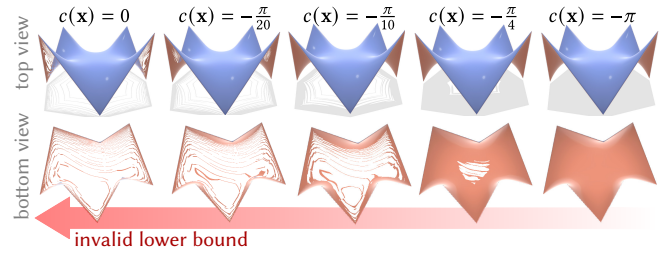
Fig. 4. Harnack tracing requires a lower bound c(\mathbf{x}) on the implicit function f(\mathbf{x}) . If c is invalid—i.e. fails to bound f —then rays may pass through the surface, yielding artifacts which become more severe as c increases (left). The artifacts are also worse for rays approaching from below ( f < f^* ), rather than above ( f > f^* ), as f takes on higher values above the surface. We describe how to obtain valid bounds in a variety of important cases.
